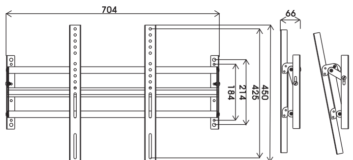
TKLA-8420 LCD TV Bracket
