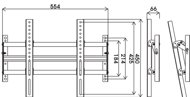
TKLA-8370 LCD TV Bracket
